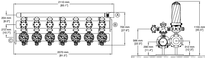
(A) Ø3" Drainage manifold (B) Ø6" Inlet manifold (C) Ø6" Outlet manifold
