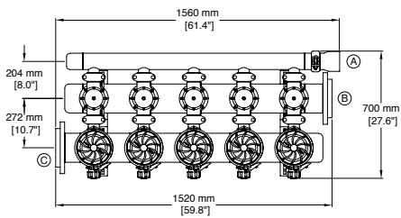
(A) Ø3" Drainage manifold (B) Ø6" Inlet manifold (C) Ø6" Outlet manifold
