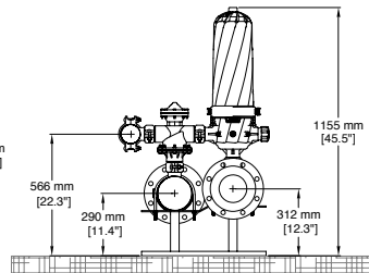
(A) Ø3" Drainage manifold (B) Ø6" Inlet manifold (C) Ø6" Outlet manifold
