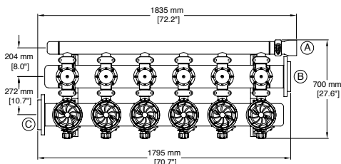
(A) Ø3" Drainage manifold (B) Ø6" Inlet manifold (C) Ø6" Outlet manifold
