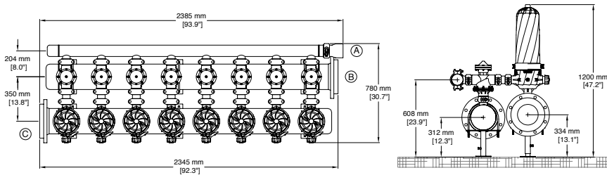
(A) Ø3" Drainage manifold (B) Ø8" Inlet manifold (C) Ø8" Outlet manifold
